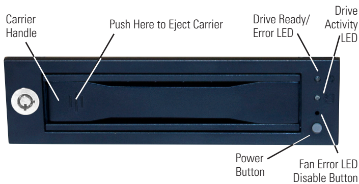
Figure 1: Front Bezel
